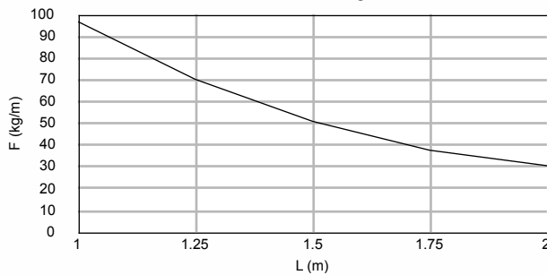
VK/VF110 Load Diagram
