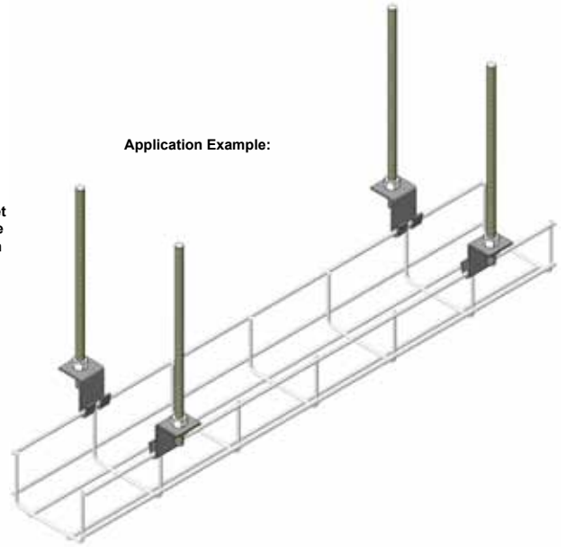
VK/VFO FOR VF Mounting Bracket Note - this bracket is only suitable for up to 200mm wide Cable Mesh
